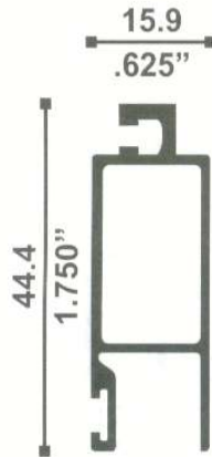
*6534 CERCO MOSQUITERO VERTICAL 0.425 Kg./m
