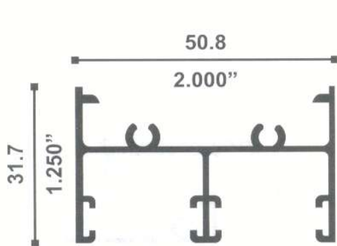
7518 JAMBA S/MOSQ. 0.590 Kg./m
